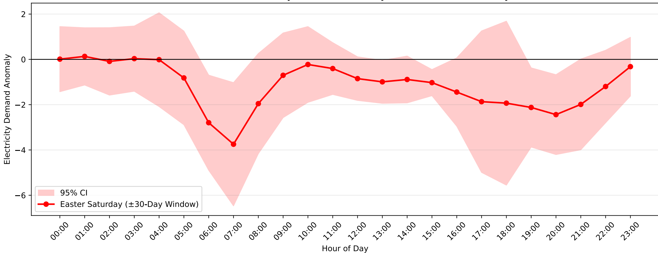
Dulwich Hill Demand Anomaly: Easter Saturday (2014–2015, \pm 30 -Day Window)
