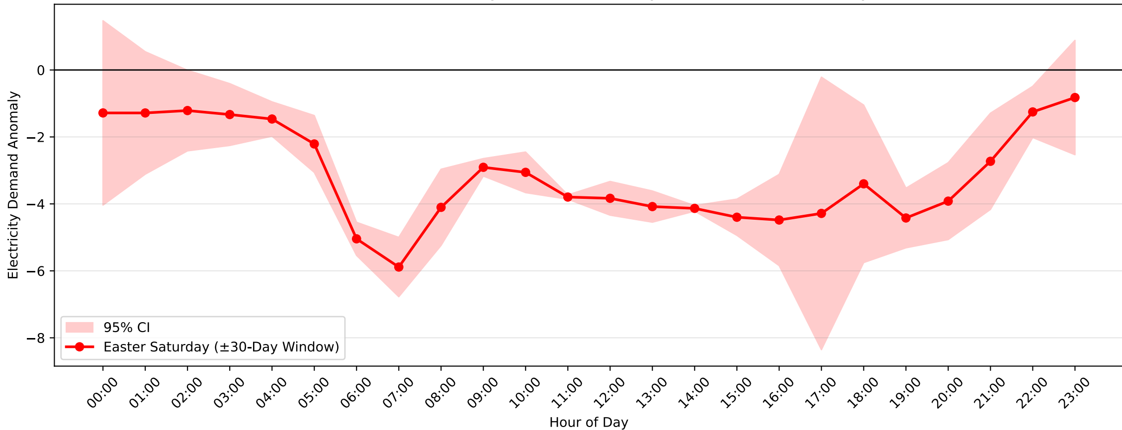
Dulwich Hill Demand Anomaly: Easter Saturday (2008–2009, \pm 30 -Day Window)
