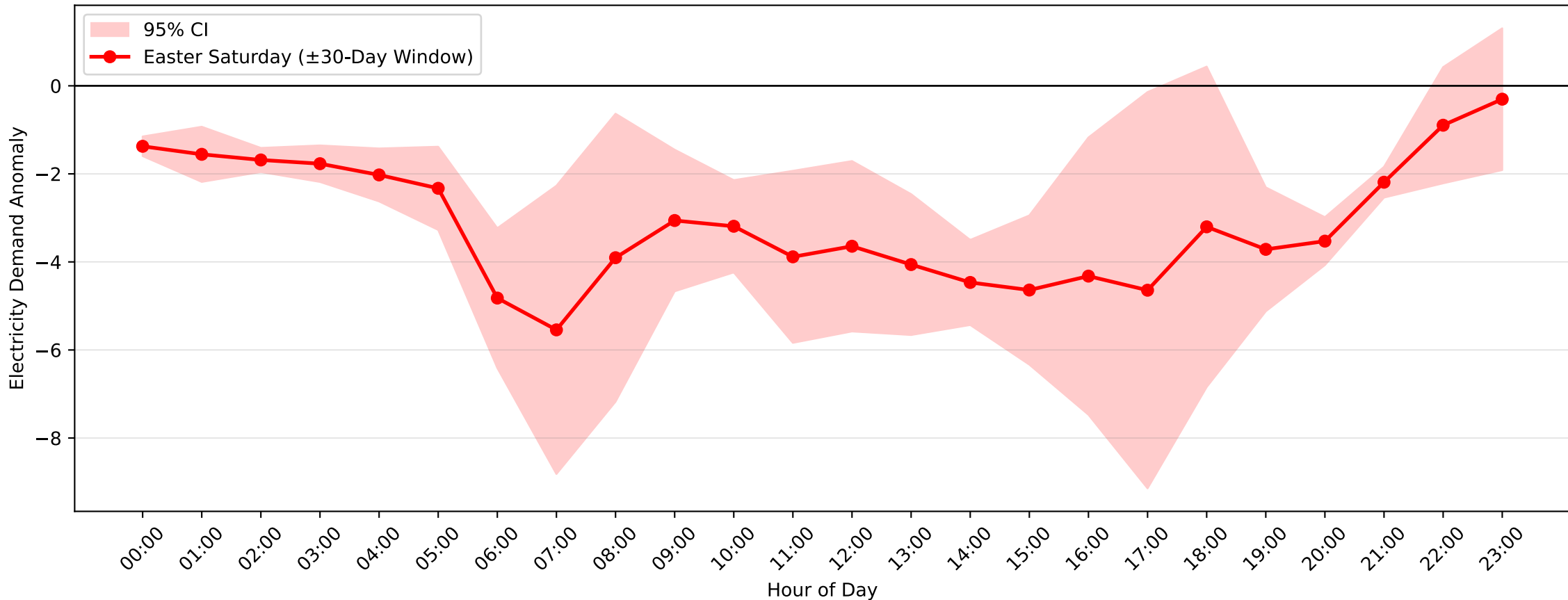
Dulwich Hill Demand Anomaly: Easter Saturday (2007–2008, \pm 30 -Day Window)
