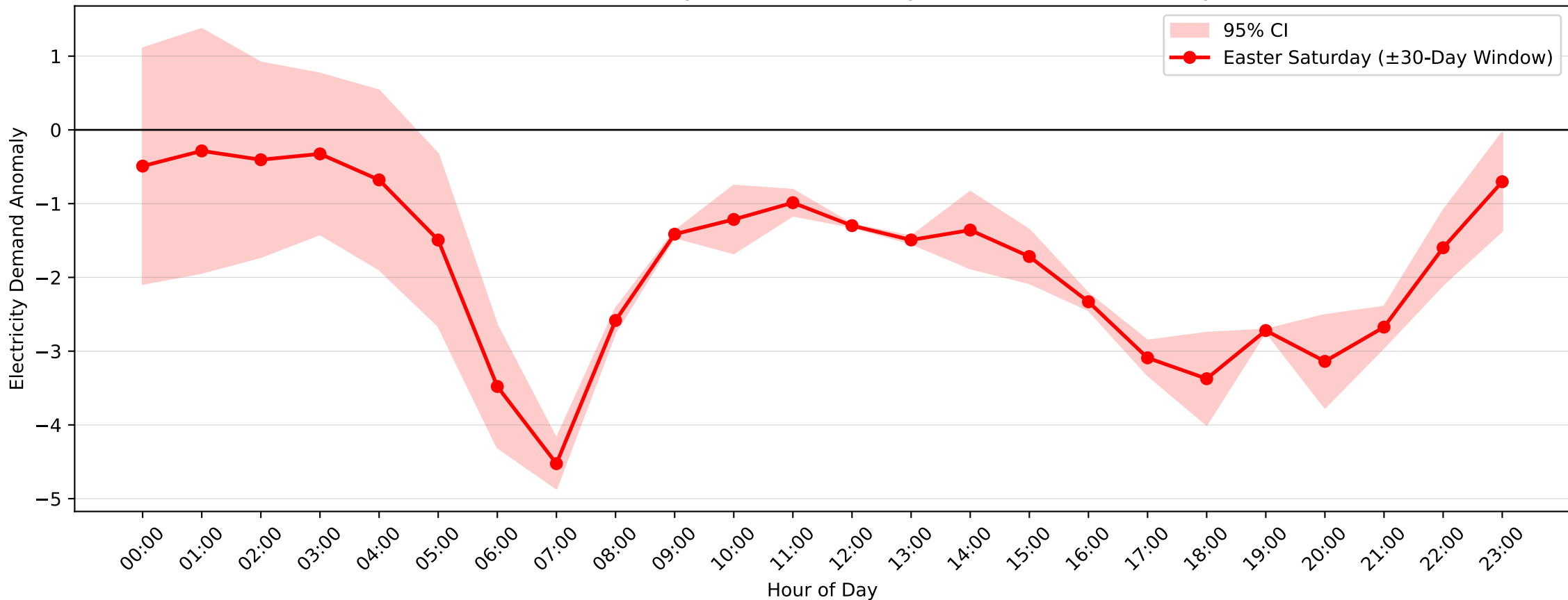
Dulwich Hill Demand Anomaly: Easter Saturday (2015–2016, \pm 30 -Day Window)
