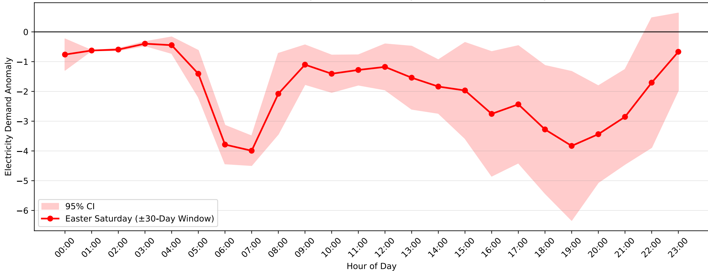
Dulwich Hill Demand Anomaly: Easter Saturday (2011-2012, \pm 30 -Day Window)
