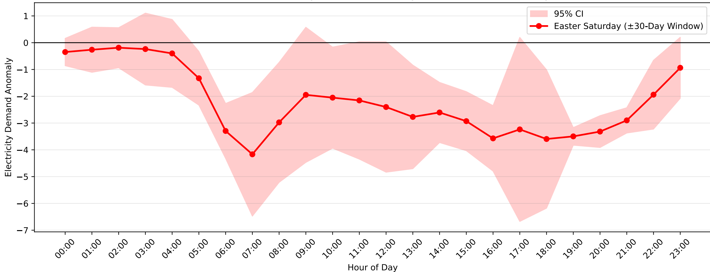
Dulwich Hill Demand Anomaly: Easter Saturday (2012-2013, \pm 30 -Day Window)
