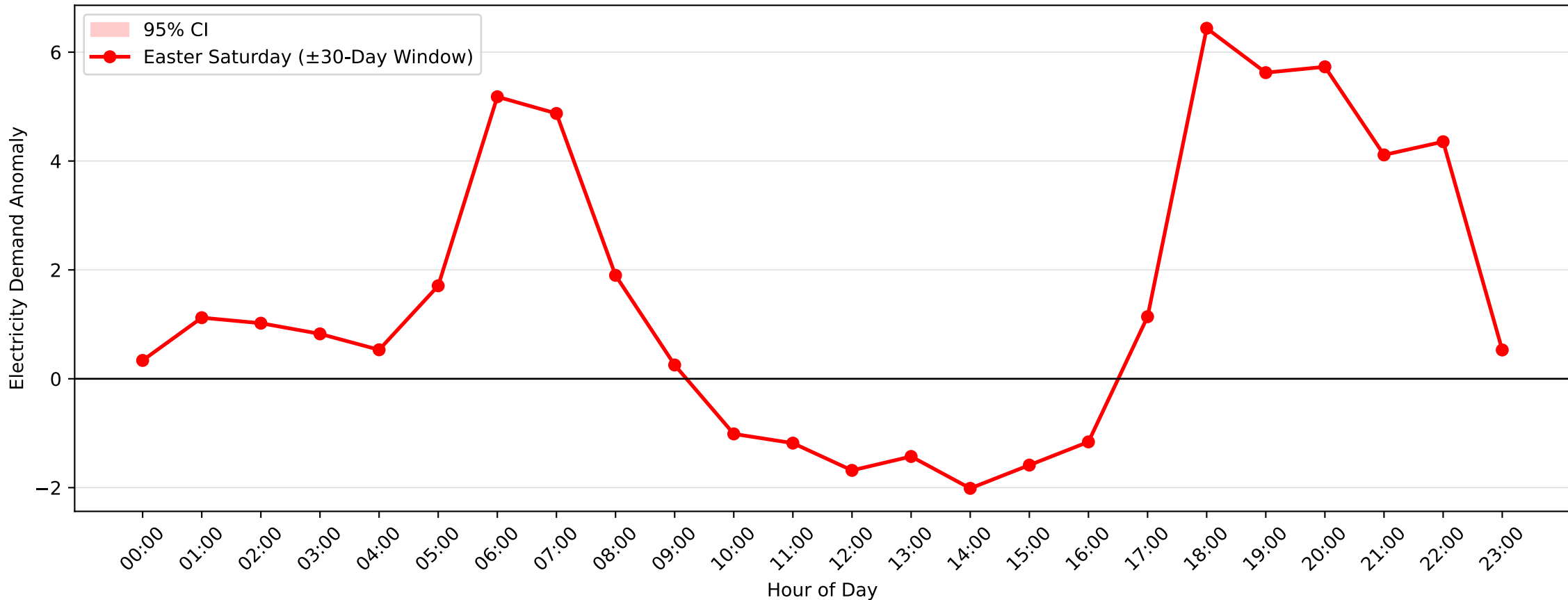
Dulwich Hill Demand Anomaly: Easter Saturday (2004–2005, \pm 30 -Day Window)
