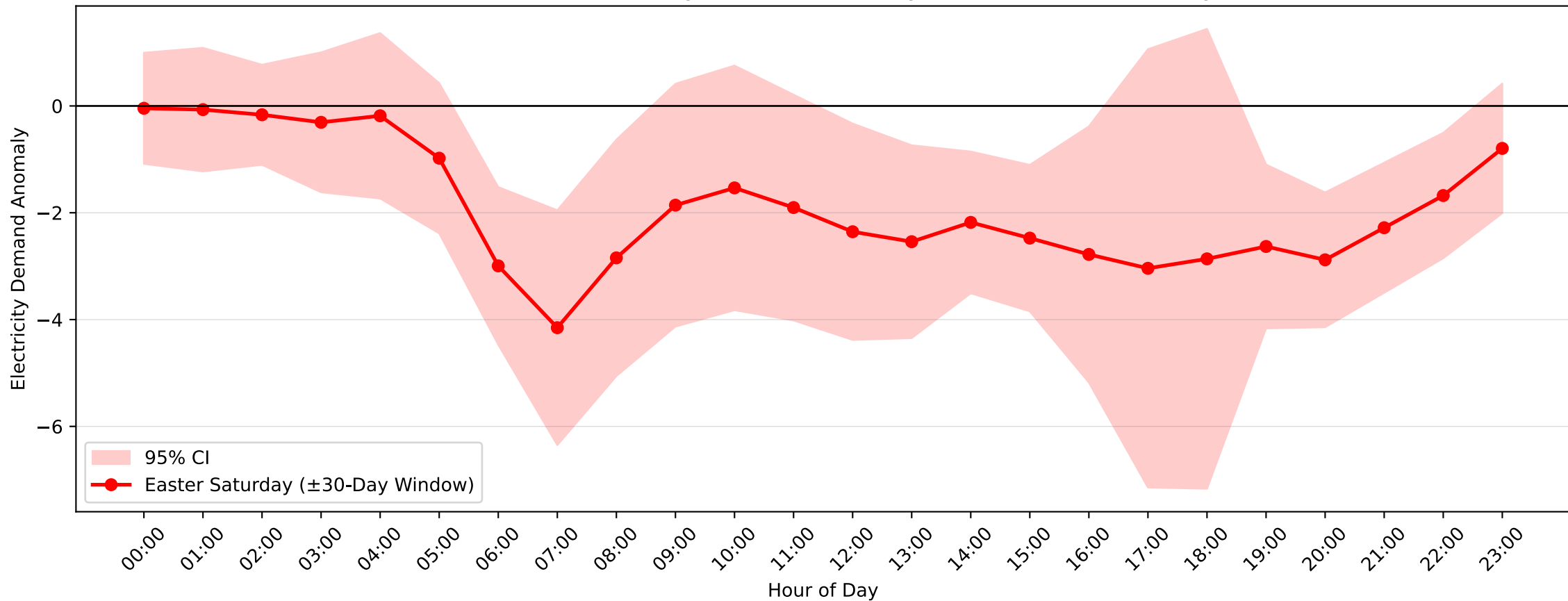
Dulwich Hill Demand Anomaly: Easter Saturday (2013–2014, \pm 30 -Day Window)
