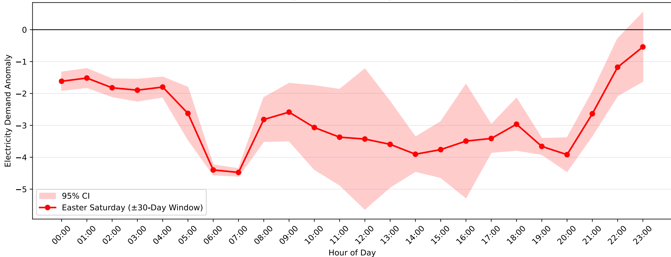
Dulwich Hill Demand Anomaly: Easter Saturday (2006–2007, \pm 30 -Day Window)
