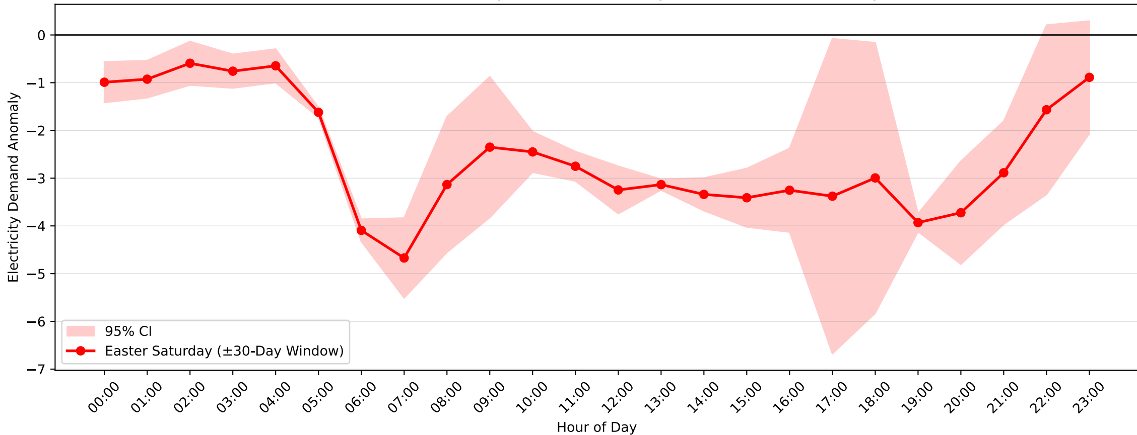
Dulwich Hill Demand Anomaly: Easter Saturday (2009–2010, \pm 30 -Day Window)
