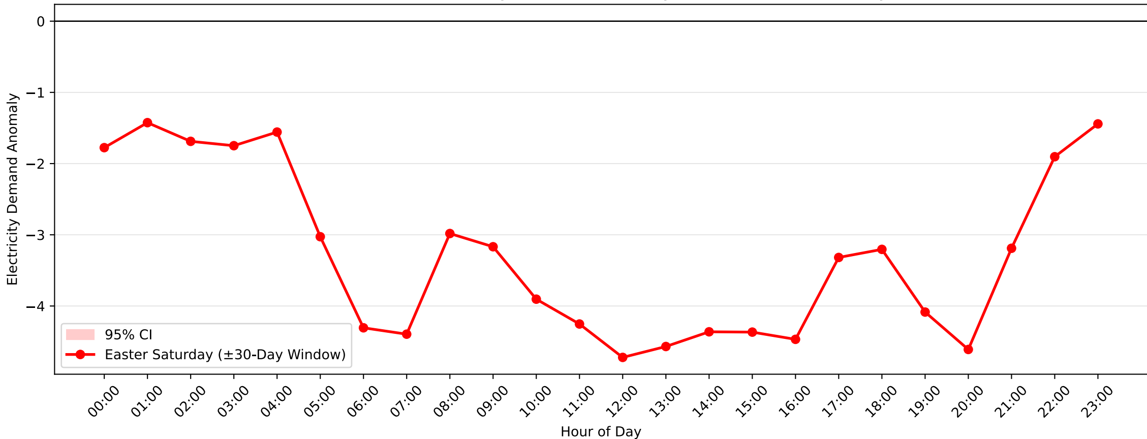
Dulwich Hill Demand Anomaly: Easter Saturday (2005–2006, \pm 30 -Day Window)
