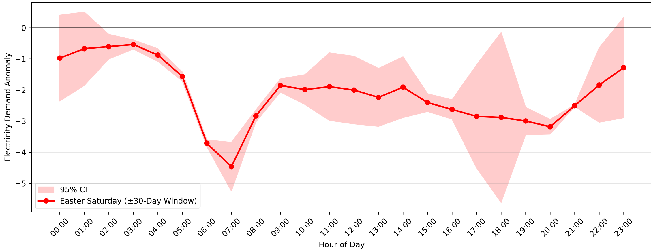
Dulwich Hill Demand Anomaly: Easter Saturday (2016–2017, \pm 30 -Day Window)
