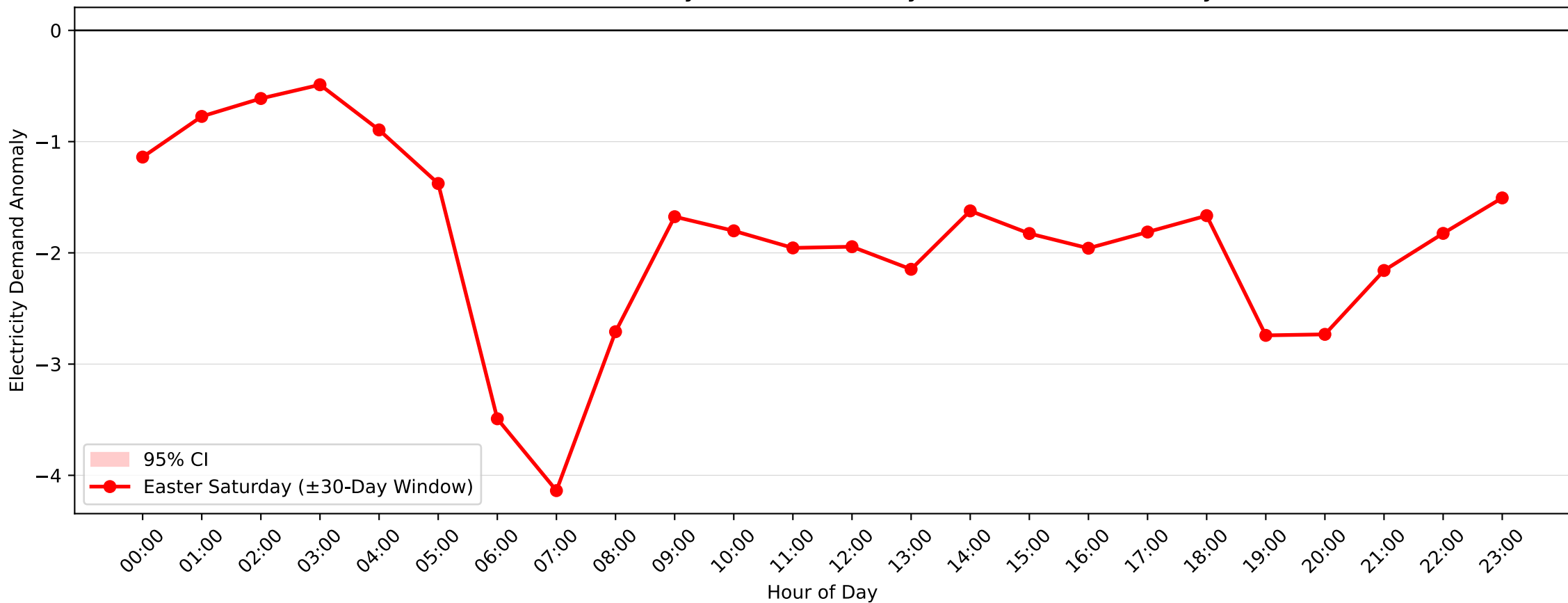
Dulwich Hill Demand Anomaly: Easter Saturday (2017-2018, \pm 30 -Day Window)
