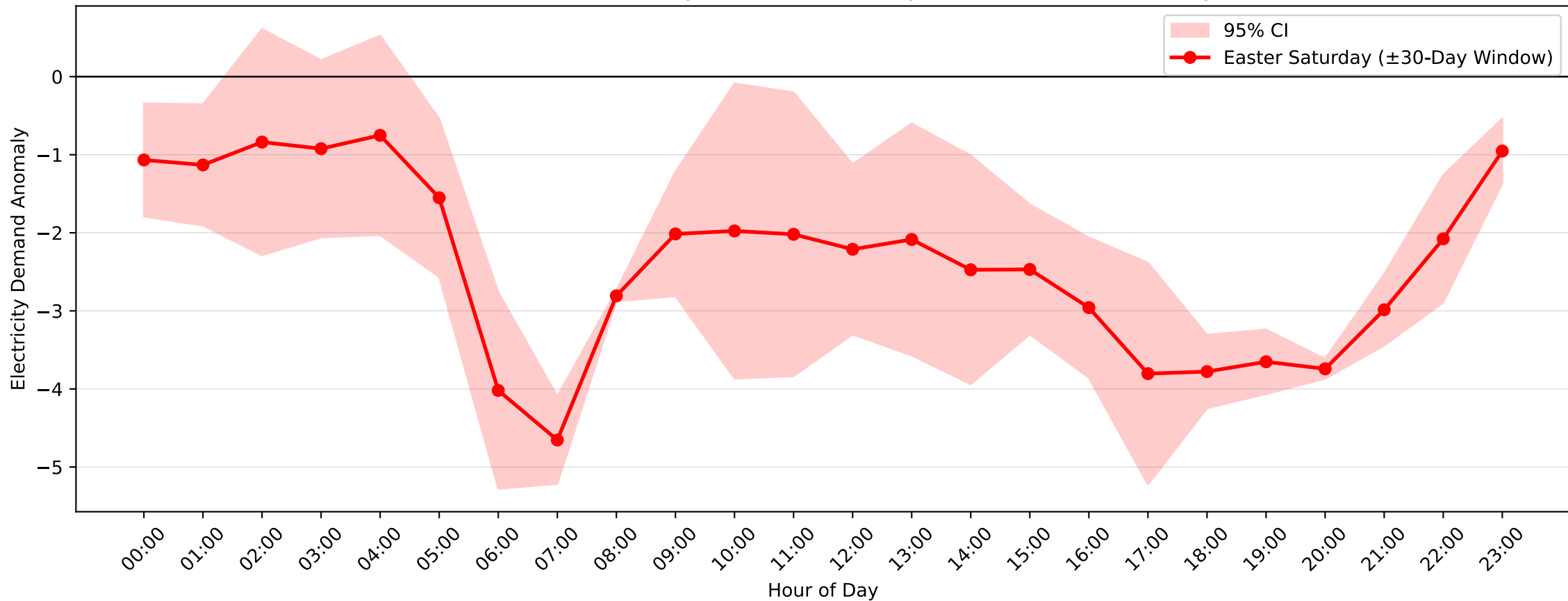
Dulwich Hill Demand Anomaly: Easter Saturday (2010-2011, \pm 30 -Day Window)
